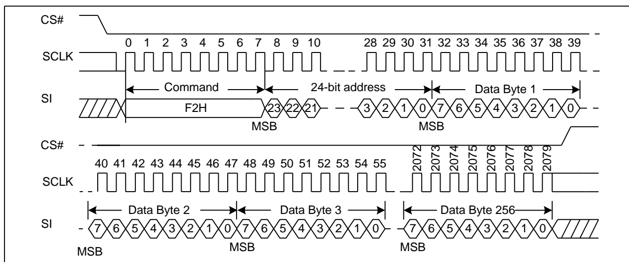
Figure 18. Fast Page Program Sequence Diagram
