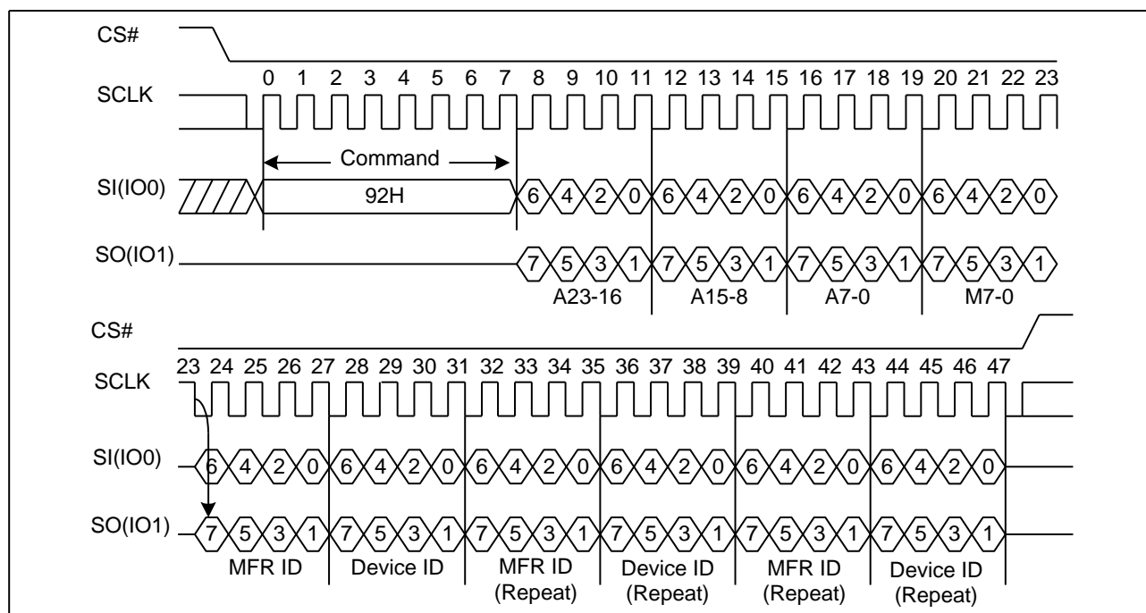
Figure 27. Dual I/O Read Manufacture ID/ Device ID Sequence Diagram
