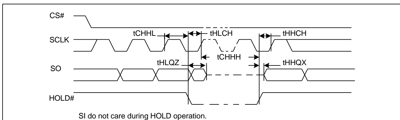
Figure 44. Hold Timing Diagram
