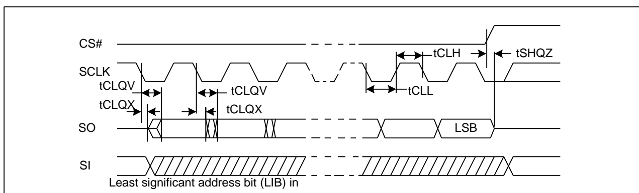
Figure 43. Output Timing Diagram
