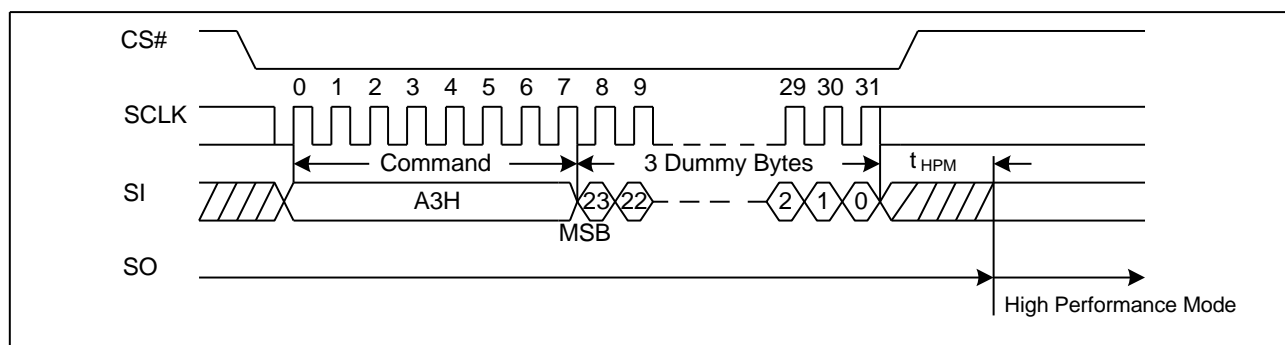
Figure 30. High Performance Mode Sequence Diagram
