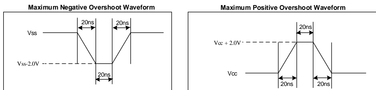
Figure 40. Maximum Negative/positive Overshoot Diagram
