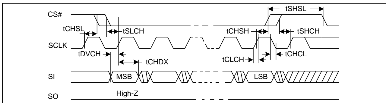
Figure 42. Serial Input Timing Diagram
