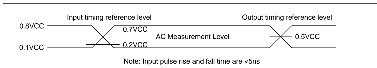
Figure 41. Input Test Waveform and Measurement Level Diagram
