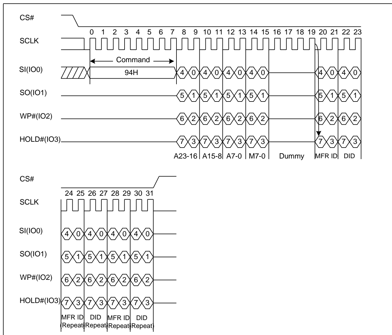
Figure 28. Quad I/O Read Manufacture ID/ Device ID Sequence Diagram
