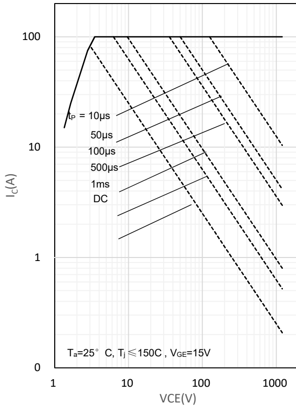
Fig. 1 FBSOA characteristics
