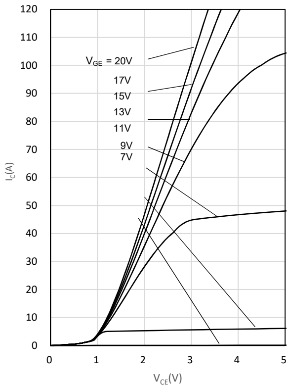
Fig. 3 Output characteristics
