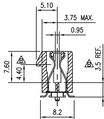
SECTION F-F
