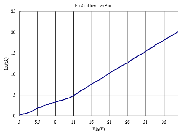
Figure 9. Shutdown Current vs. V_{IN}
