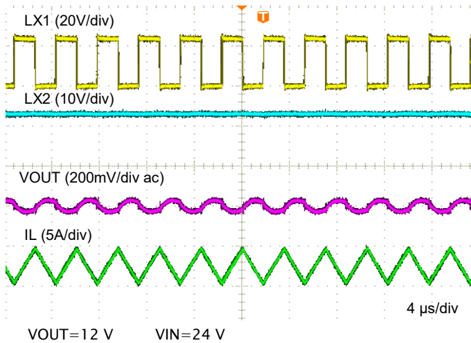
Figure 16. Forced CCM Operation (Buck)
