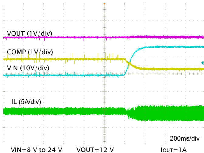
Figure 23. Line Transient
