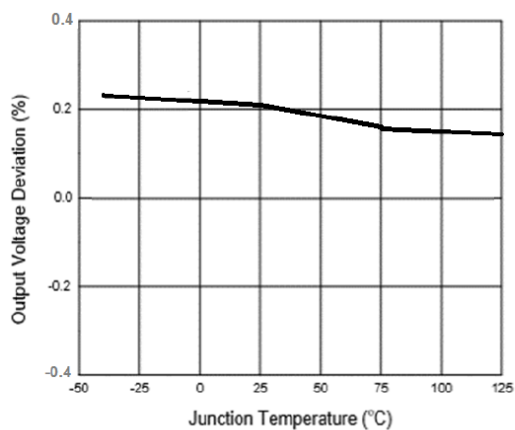
Load Regulation vs. Junction Temperature
