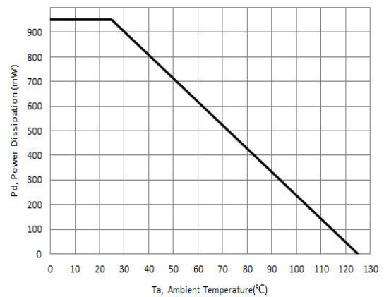
Derating Curve(S-LR117DD)
