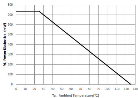
Derating Curve(S-LR117DS)
