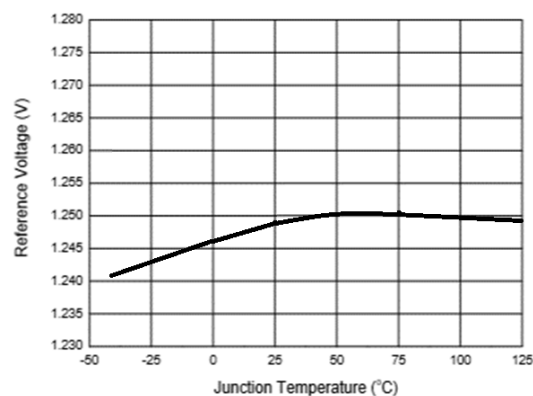
Reference Voltage vs. Junction Temperature
