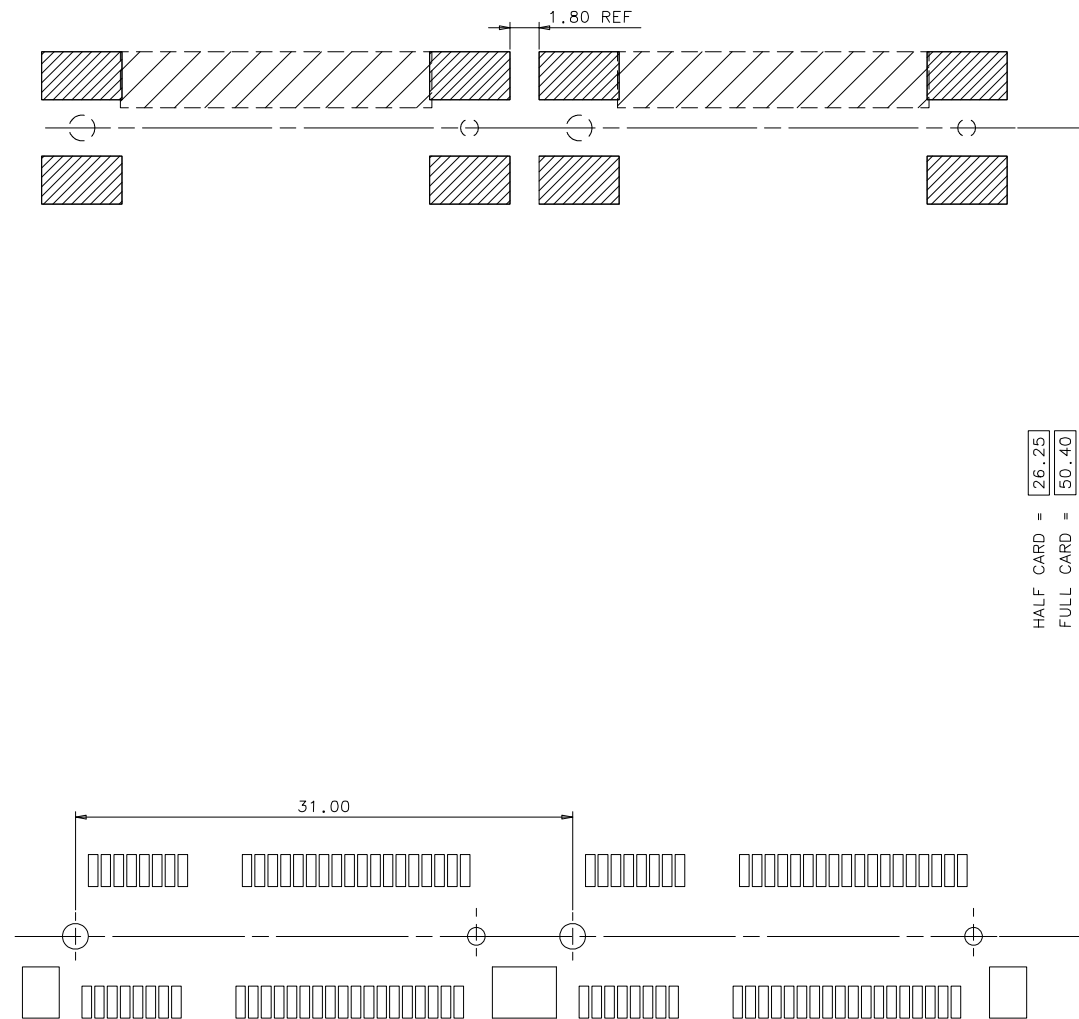
RECOMMENDED PCB LAYOUT (SIDE BY SIDE)
