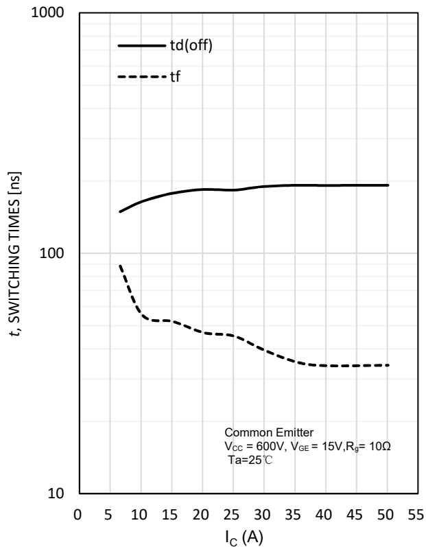
Fig. 6 Turn-off time vs. collector current
