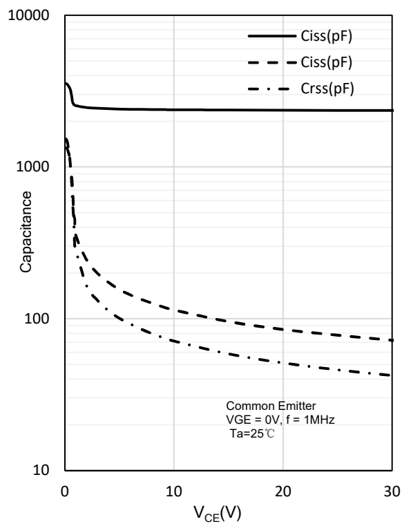
Fig. 10 Capacitance characteristics
