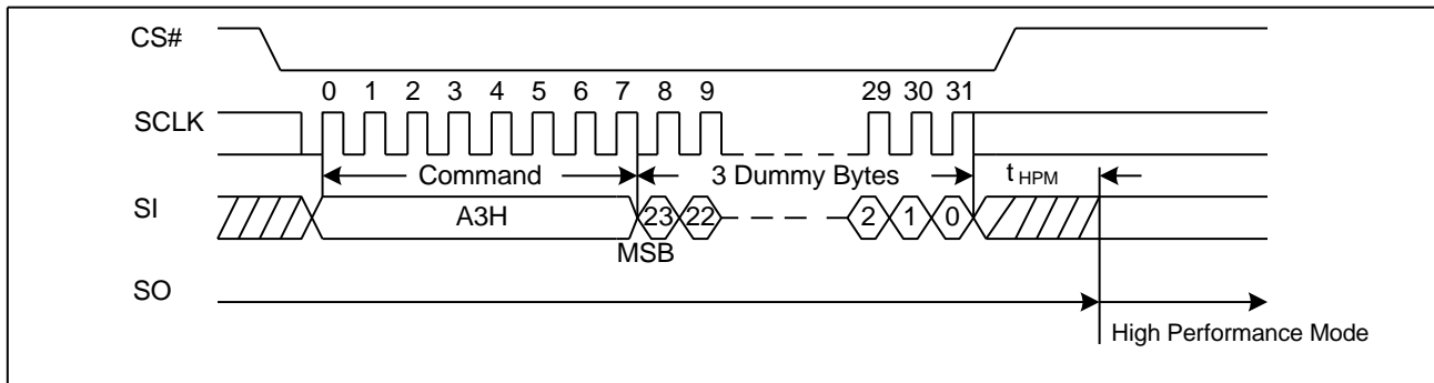
Figure 30. High Performance Mode Sequence Diagram
