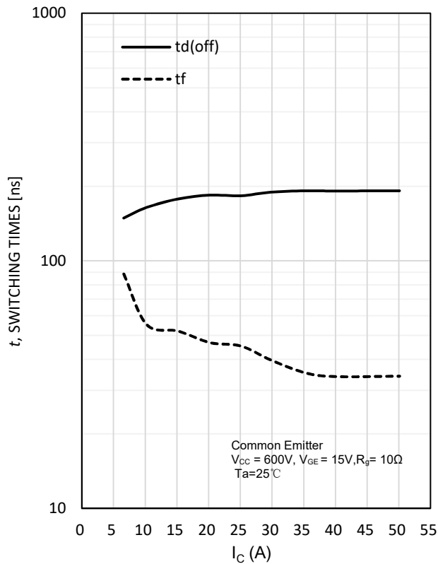
Fig. 4 Turn-off time vs. collector current
