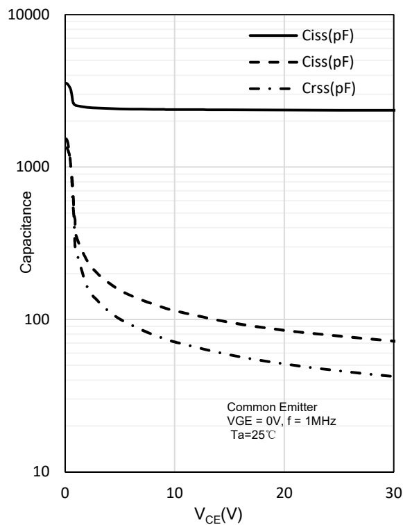
Fig. 8 Capacitance characteristics
