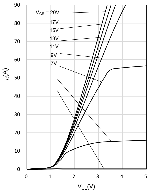
Fig. 1 Output characteristics
