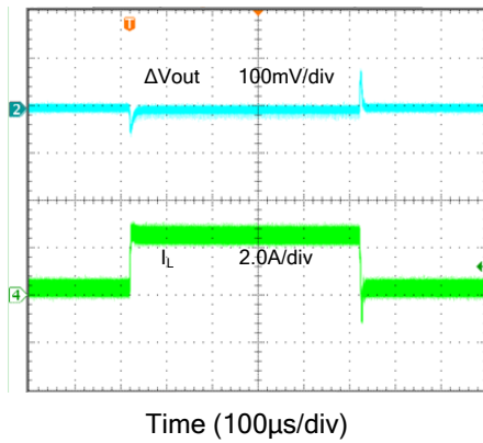
Load Transient ( V_{IN}=5.0V , V_{OUT}=1.8V , I_{LOAD}=0.25-2.5A )
