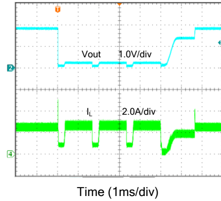
Hard Short Protection ( V_{IN}=5.0V , V_{OUT}=1.8V , 2.5A to Short)
