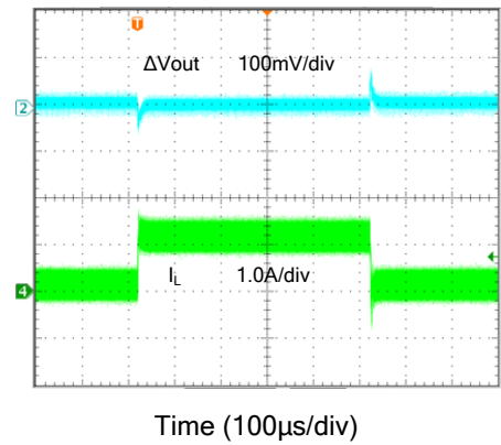
Load Transient ( V_{IN}=5.0V , V_{OUT}=1.8V , I_{LOAD}=0-1.25A )
