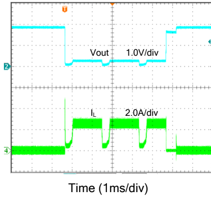
Hard Short Protection ( V_{IN}=5.0V , V_{OUT}=1.8V , Null Load To Short)
