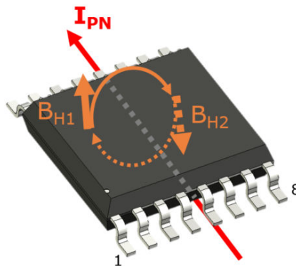
Figure 10 Current polarity (PG-TDSO-16)
