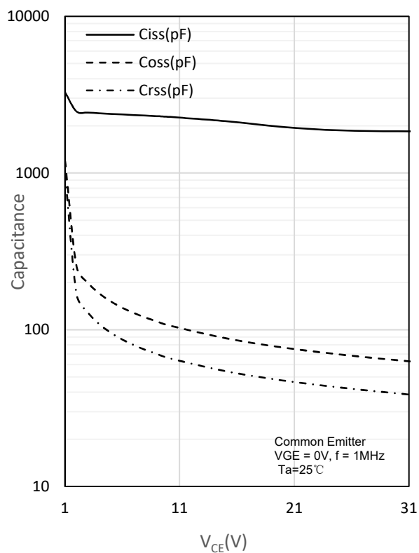
Fig. 10 Capacitance characteristics
