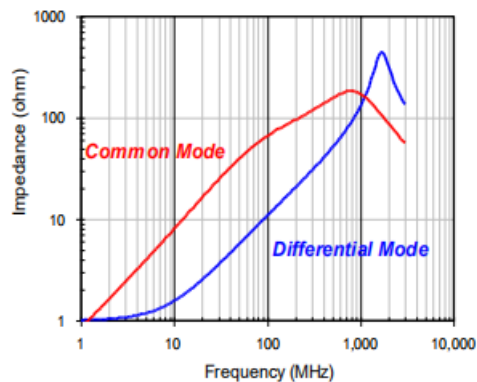
IMPEDANCE vs. FREQUENCY CHARACTERISTICS
