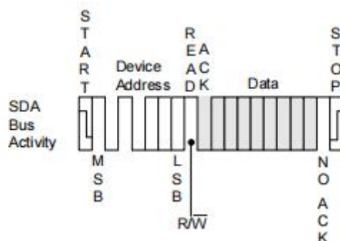
Figure8.Current Address Read
