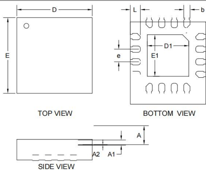
QFN3.0X3.0X0.75-16L产品外形图
