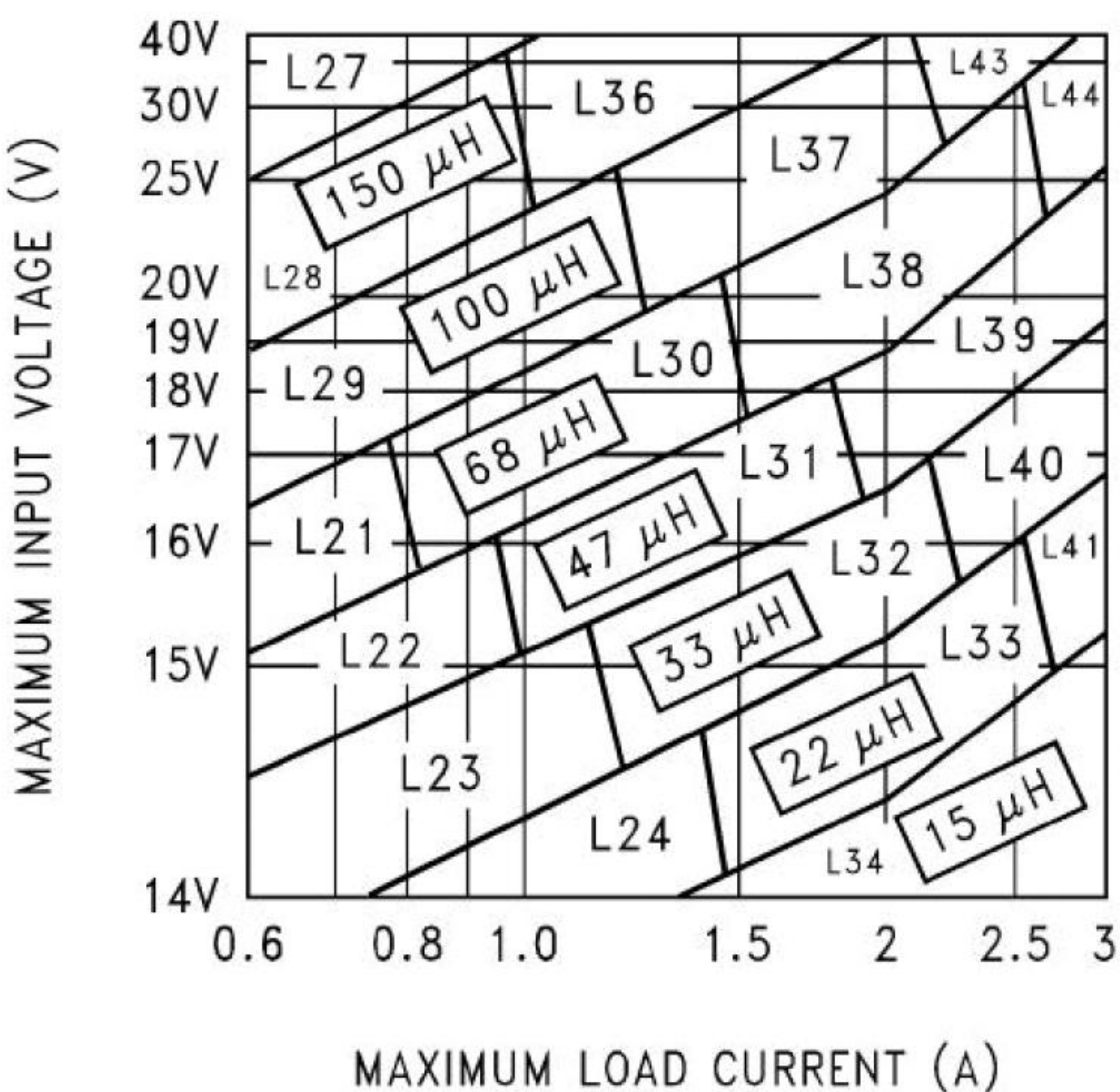
LM2596HV-12
