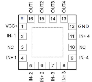
QFN-16 3*3
