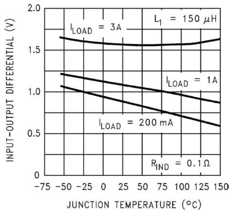
Dropout Voltage
