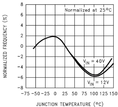
Oscillator Frequency
