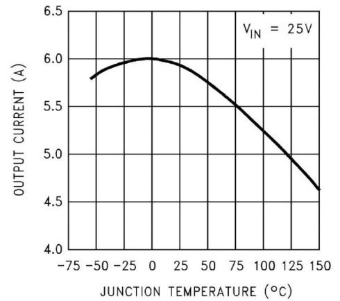
Current Limit
