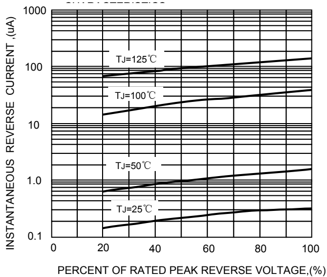
FIG.3-TYPICAL REVERSE
