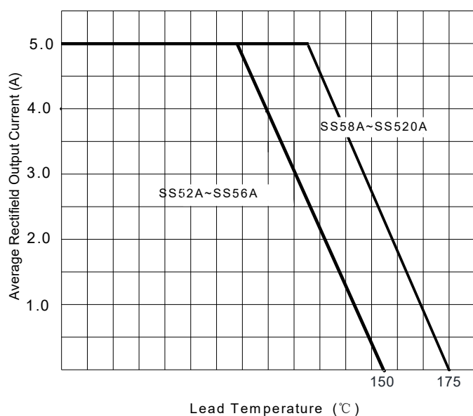
FIG1: Io-TL Curve
