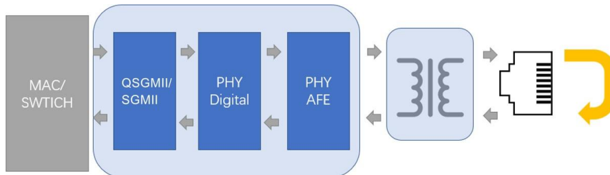
Figure 10. External Loopback
