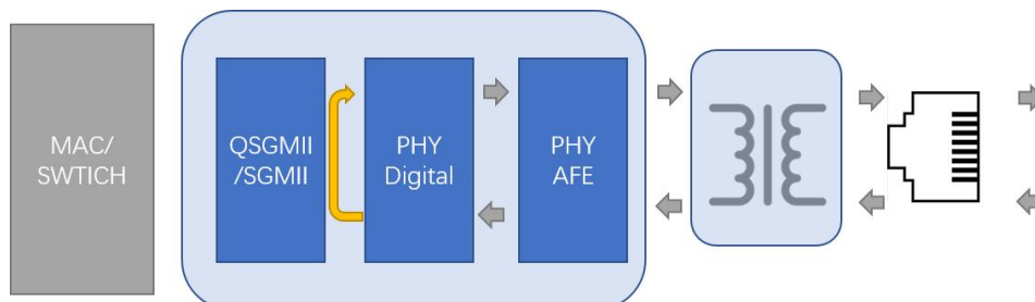
Figure 11. Remote PHY Loopback
