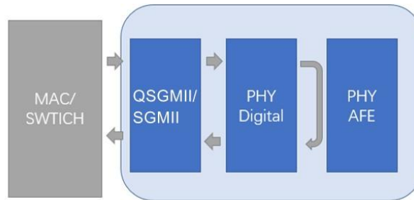
Figure 9. Digital Loopback
