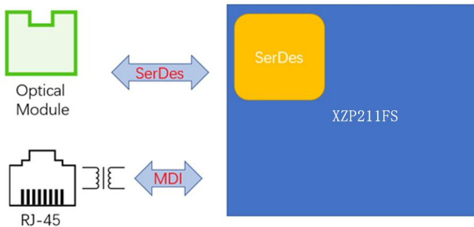
Figure 7. Fiber to UTP Application
