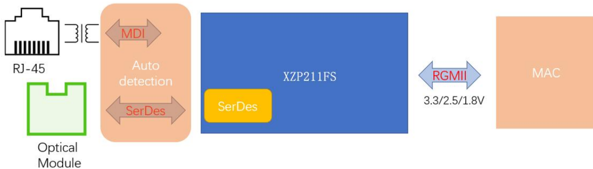
Figure 5. UTP/Fiber to RGMII Application
