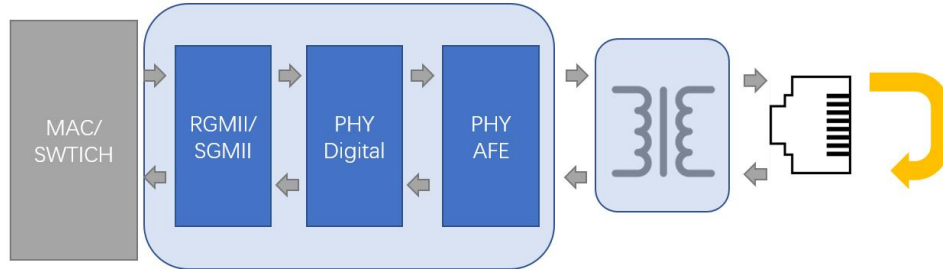
Figure 9. External Loopback
