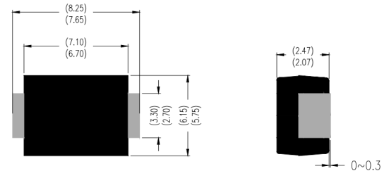
SMC/DO-214AB
