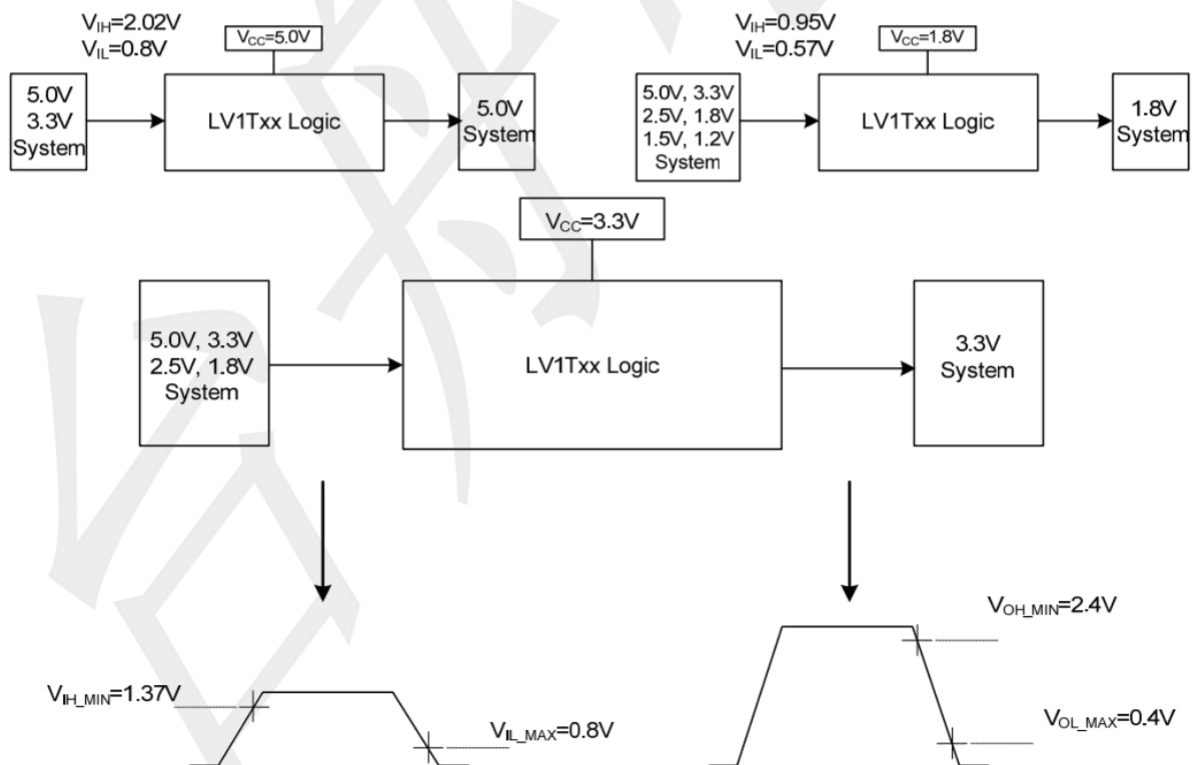
Switching Thresholds for 1.8V~3.3V Translation
