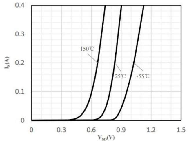
Body-Diode Characteristics
