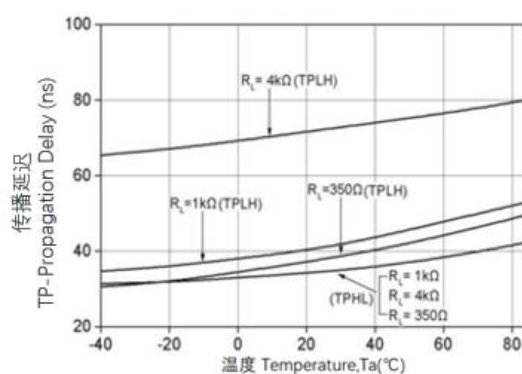
Figure 8. Switching Time vs Temperature
