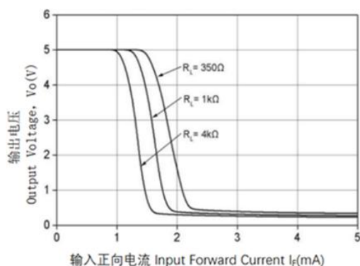
Figure 5. Output Voltage vs Forward Current Temperature
