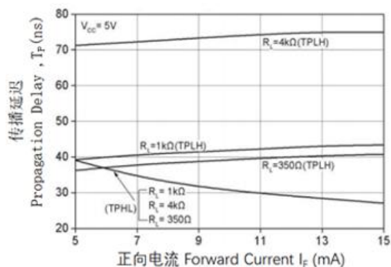
Figure 7. Switching Time vs Forward Current
