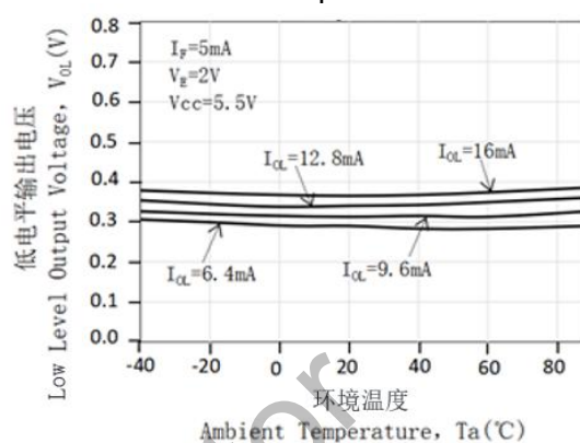
Fig.2 Low Level Output Voltage vs Ambient Temperature
