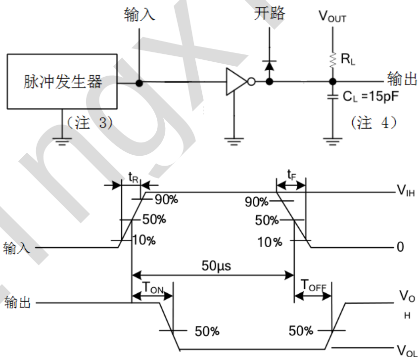
8. t_{ON}, t_{OFF}
