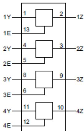
Figure 1. Functional diagram
