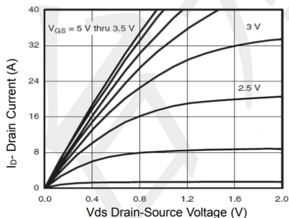
Figure 5 Output Characteristics
