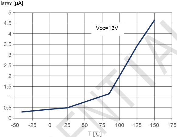
Standby current
