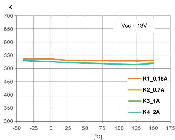
I OUT /I SENSE vs. T A
