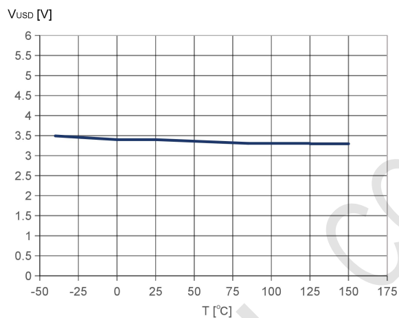
Undervoltage shutdown
