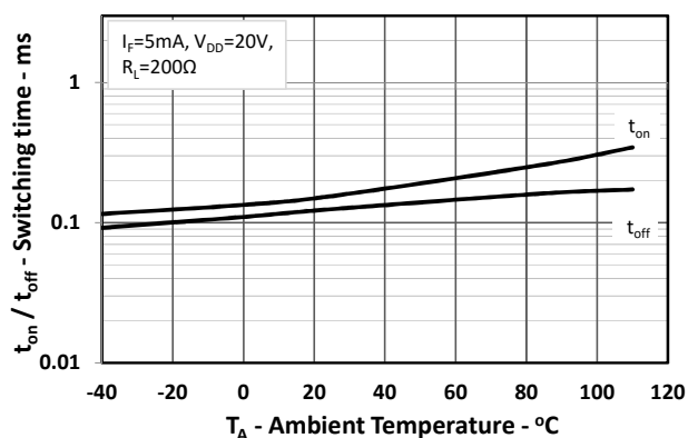
Fig. 7 Switching time vs. Ambient Temperature
