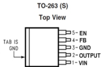
TO263-5L (LM2576S)
