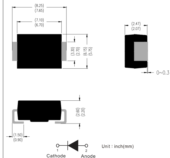
SMC/DO-214AB
