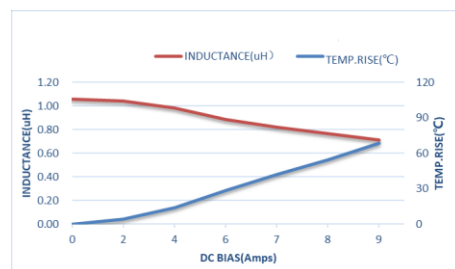
ZEPIM303015D-1R0M
