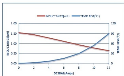
ZEPIM303015D-1R5M
