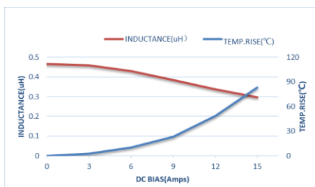
ZEPIM303015D-R47M
