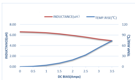
ZEPIM303015D-6R8M
