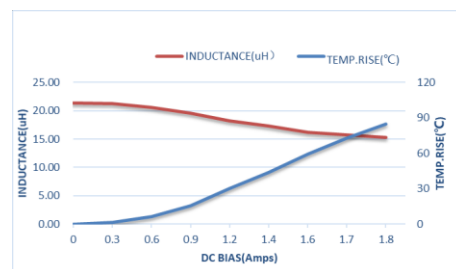
ZEPIM303015D-220M
