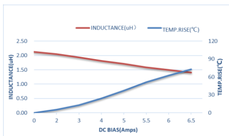
ZEPIM303015D-2R2M
