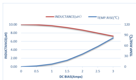
ZEPIM303015D-100M
