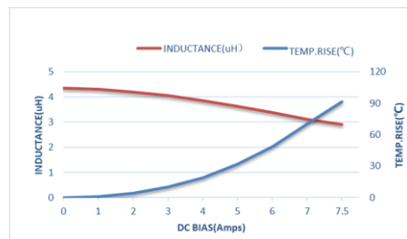
ZETC404020S-4R7MT-LF
