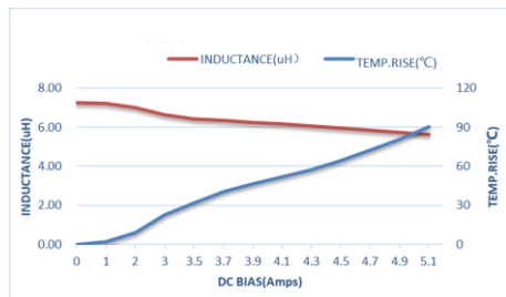
ZETC404020S-6R8MT-LF
