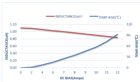
ZETC404020S-1R0MT-LF
