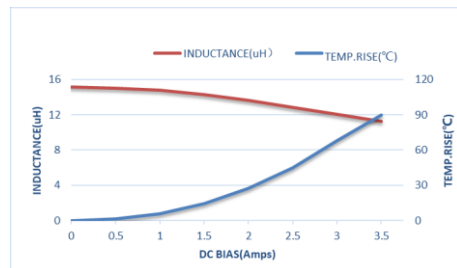
ZETC404020S-150MT-LF
