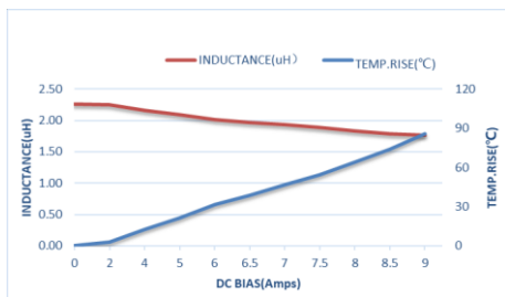
ZETC404020S-2R2MT-LF
