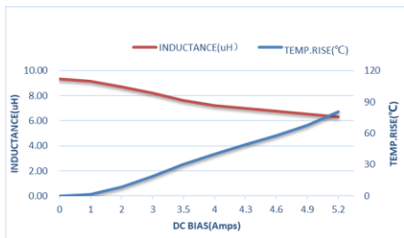
ZETC404020S-100MT-LF
