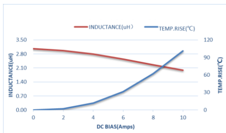
ZETC404020S-3R3MT-LF
