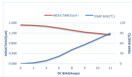
ZETC404020S-1R5MT-LF
