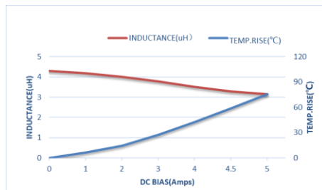
ZETC303018D-4R7MT-LF
