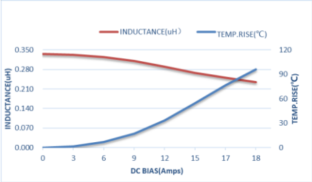
ZETC303020DR33MBT-LF
