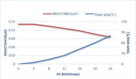
ZETC303020DR15MBT-LF
