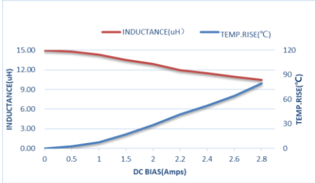
ZETC303020D150MBT-LF
