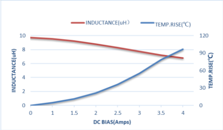
ZETC303020D100MBT-LF
