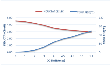
ZETC303020D4R7MBT-LF
