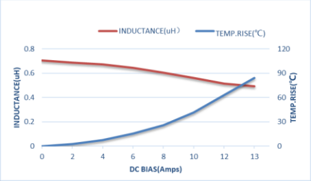
ZETC303020DR68MBT-LF
