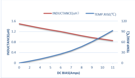
ZETC303020D1R5MBT-LF
