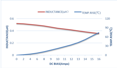
ZETC303020DR50MBT-LF
