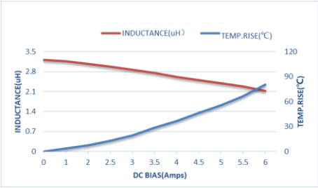
ZETC303020D3R3MBT-LF
