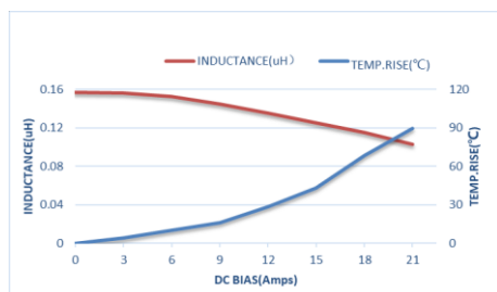
ZETC303015D-R15MT-LF
