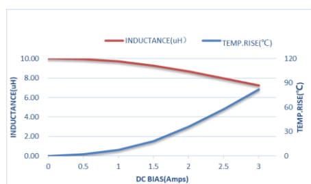
ZETC303015D-100MT-LF
