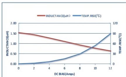
ZETC303015D-1R5MT-LF
