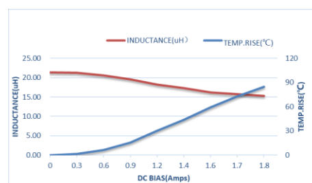
ZETC303015D-220MT-L
