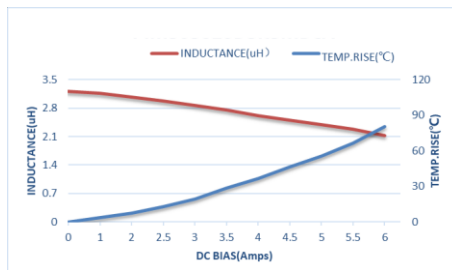
ZETC303020D3R3MBT-LF
