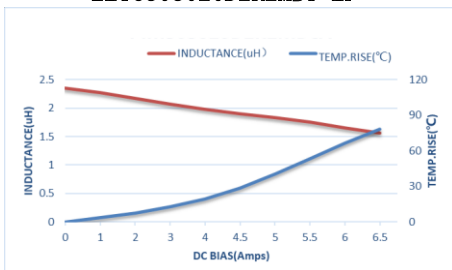
ZETC303020D2R2MBT-LF
