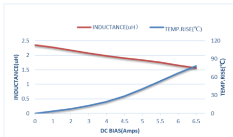
ZETC303020D-2R2MT-LF
