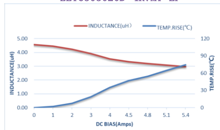
ZETC303020D-4R7MT-LF
