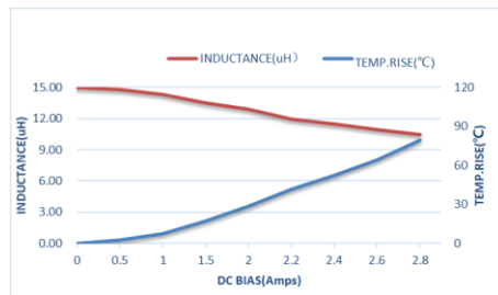
ZETC303020D-150MT-LF
