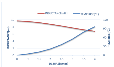
ZETC303020D-100MT-LF
