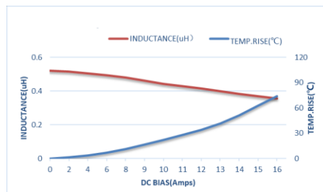
ZETC303020D-R50MT-LF
