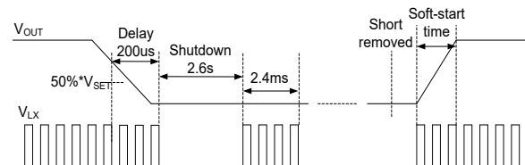
Fig. 6 Description of Short-circuit Protection
