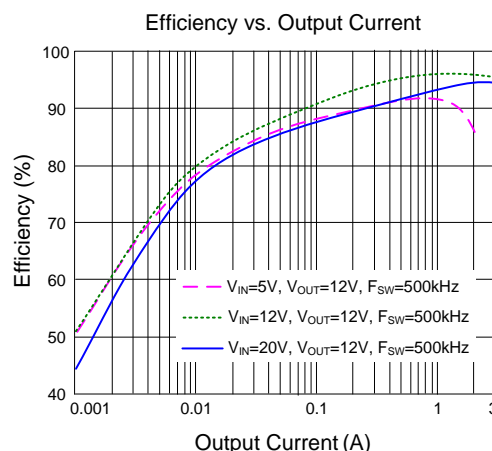
Fig.2 Efficiency vs. Output Current
