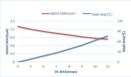
ZET-CORE-303018DT1R5MBCA
