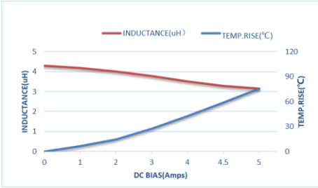
ZET-CORE-303018DT4R7MBCA
