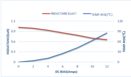
ZET-CORE-303018DT1R0MBCA
