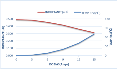
ZET-CORE-303018DTR47MBCA
