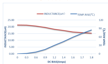
ZEPIM303015T220MLF
