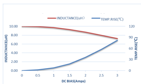
ZEPIM303015T100MLF
