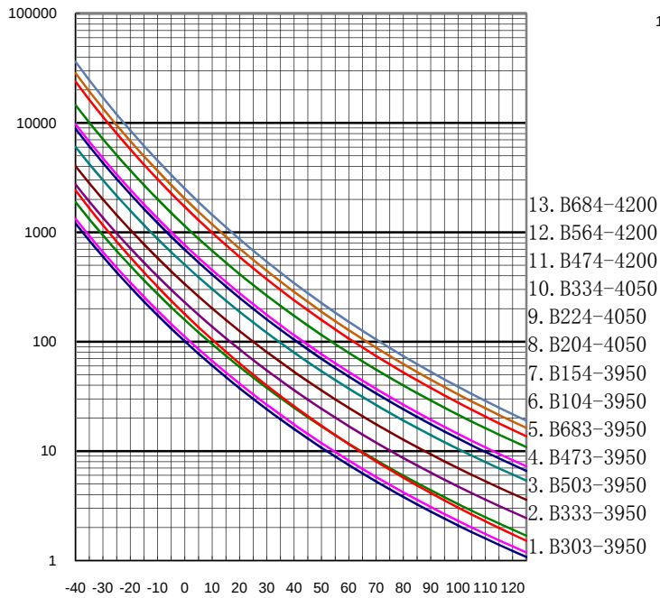
CMFB303-684
