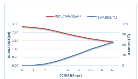
ZETC404012S3R3MBT-LF
