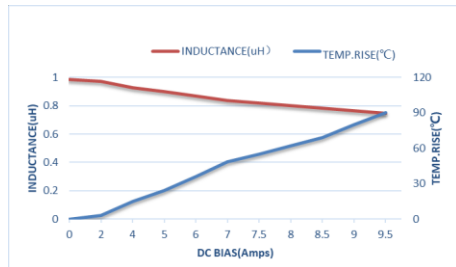
ZET-CORE-404012ST1R0MBCA
