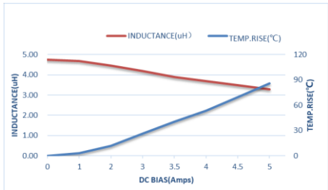
ZET-CORE-404012ST4R7MBCA
