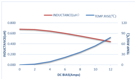
ZET-CORE-404012STR68MBCA
