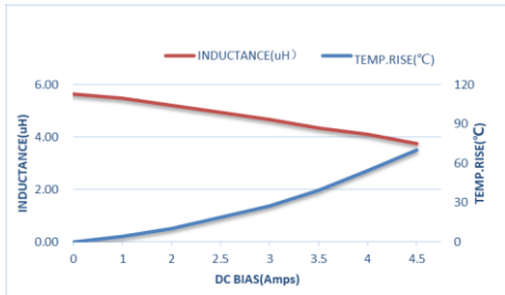
ZET-CORE-404012ST5R6MBCA
