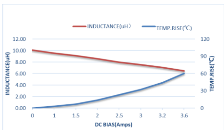
ZET-CORE-404012ST100MBCA
