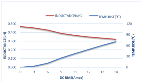
ZET-CORE-404012STR47MBCA
