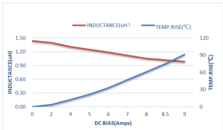
ZET-CORE-404012ST1R5MBCA
