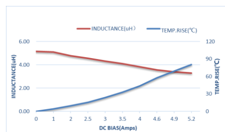
ZET-CORE-303015DT4R7MBCA
