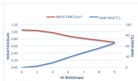
ZET-CORE-303015DT1R0MBCA
