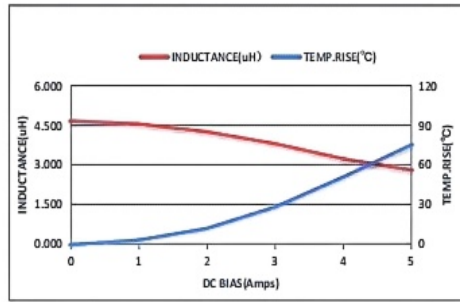
ZETC404010S4R7MBT-LF
