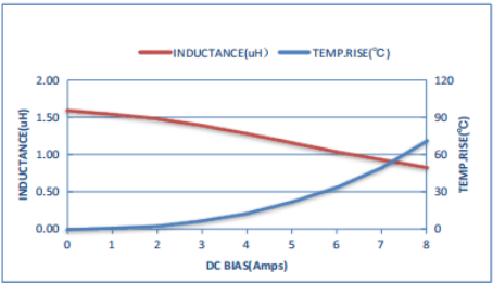
ZEP1M303012D-1R5M
