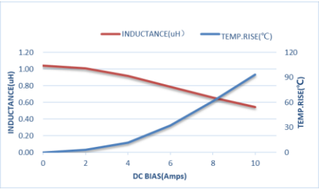
ZEP1M303012D-1R0M
