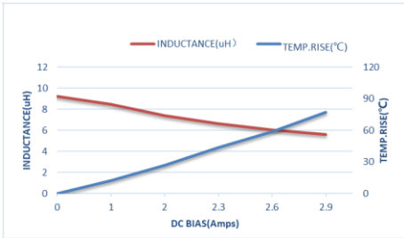
ZEP1M303012D-100M
