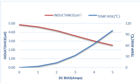
ZEP1M303012D-4R7M
